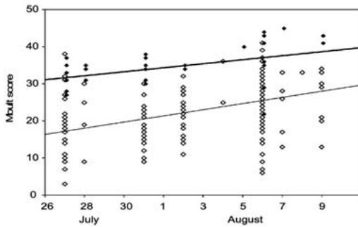
Figure 2. Regression between primary molt score and days (day 1 = 1 July) for second-year (black squares, thick line) and adult (open squares, thin line) Black-headed Gulls caught during autumn migration in Rewa between 27 July and 9 August in years 1992-1995. Slopes of regression lines differ significantly (ANCOVA, F_{1,214} = 4.7 , P = 0.003 ).
